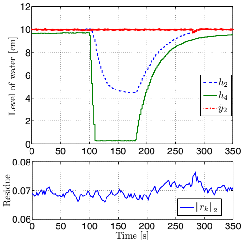
Figure 7: Results for the replay attack performed against sensor 2 from t \approx 100 s to t \approx 280 s. Additionally, the attacker opens the tap of tank 4 at t \approx 100 s and closes it at t \approx 180 s.
